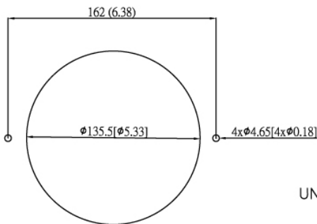
Mountion Panel Cutout Outlet Side & Inlet Side
