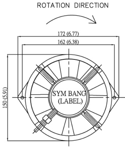
Mountion Panel Cutout Outlet Side & Inlet Side
