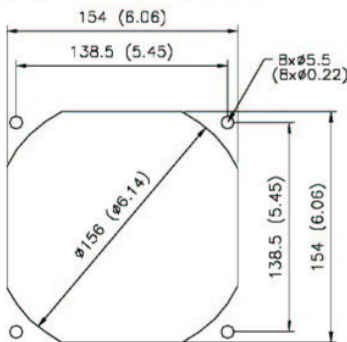
Mountion Panel Cutout Outlet Side & Inlet Side
