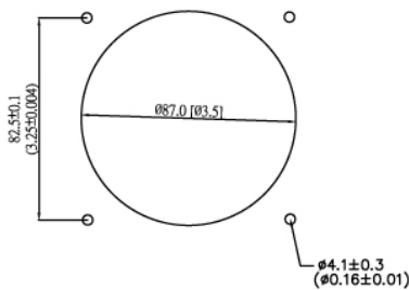
Mountiom Panel Cutout Outlet Side & Inlet Side
