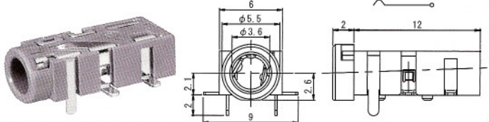
No.M03-A10C0 (3.5φ-5極) 5-CONDUCTOR MINIATURE JACK FOR P.C.B
