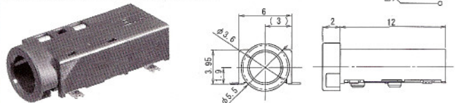
No.MJ-7835-5 (3.5φ-4極) No.MJ-7835-6 (3.5φ-4極) 4-CONDUCTOR MINIATURE JACK FOR P.C.B
