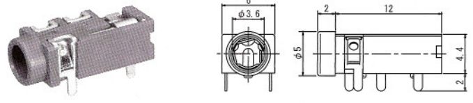
No.MJ-8435 (3.5φ-3極) 3-CONDUCTOR MINIATURE JACK FOR P.C.B STEREO
