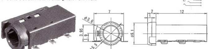
No.M03-A50C0 (3.5φ-6極) 6-CONDUCTOR MINIATURE JACK FOR P.C.B
