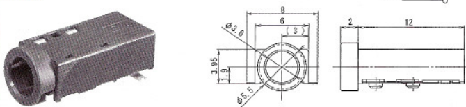
No.M03-A40C0 (3.5φ-4極) 4-CONDUCTOR MINIATURE JACK FOR P.C.B
