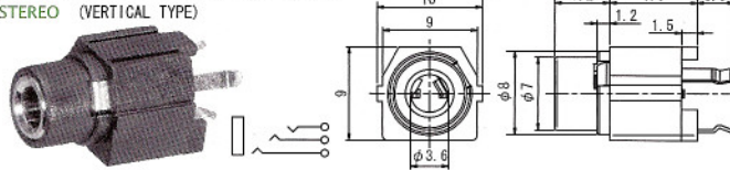
No.M03-A30C0 (3.5φ-3極) 3-CONDUCTOR MINIATURE JACK FOR P.C.B STEREO
