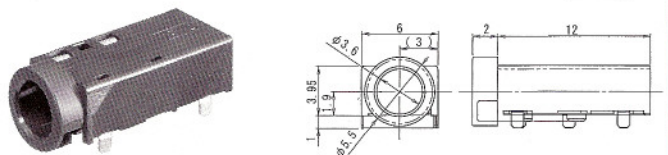
No.M03-A41A0 (3.5φ-4極 防水型) 4-CONDUCTOR MINIATURE JACK FOR P.C.B (WATER PROOF)
