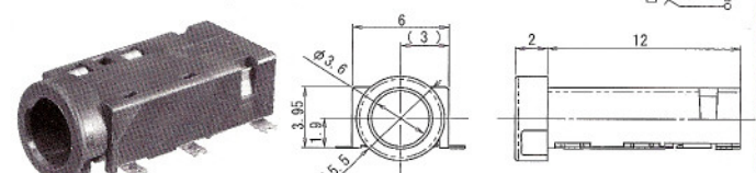
No.M03-A10C0 (3.5φ-5極) 5-CONDUCTOR MINIATURE JACK FOR P.C.B
