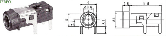
No.M03-A30A0 (3.5φ-3極) 3-CONDUCTOR MINIATURE JACK FOR P.C.B STEREO
