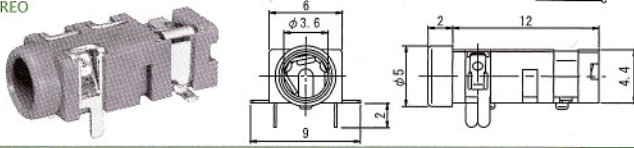
No.MJ-9135 (3.5φ-3極 縦型) 3-CONDUCTOR MINIATURE JACK FOR P.C.B STEREO (VERTICAL TYPE)
