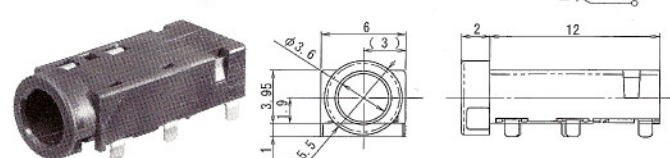
No.M03-A10A0 (3.5φ-5極) 5-CONDUCTOR MINIATURE JACK FOR P.C.B
