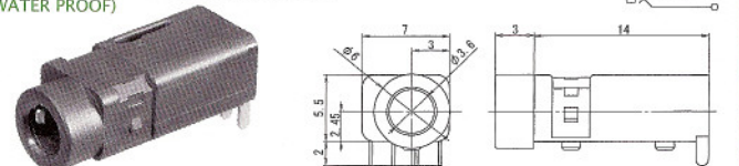
No.MJ-9935 (3.5φ-4極) 4-CONDUCTOR MINIATURE JACK FOR P.C.B
