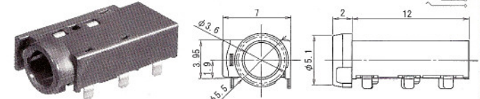
No.M19-A11Y0 (3.5φ-6極) 6-CONDUCTOR MINIATURE PLUG FOR MOLDING
