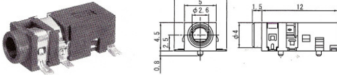
No.MJ-8635 (3.5φ-3極) 3-CONDUCTOR MINIATURE JACK FOR P.C.B STEREO
