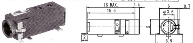
No.M03-A10A0 (3.5φ-5極) 5-CONDUCTOR MINIATURE JACK FOR P.C.B
