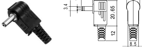
No.MP-121WN 3.4 × 1.4 RIGHT ANGLE DC PLUG (DC12V 0.5A)
