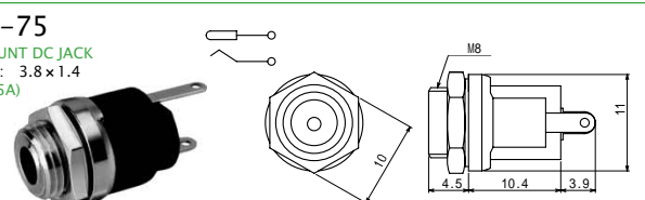
No.MJ-099N/3.8 DC INLINE JACK PLUG TYPE: 3.8 × 1.4 (DC12V 0.5A)
