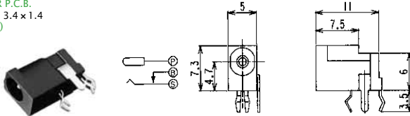
No.MJ-441DJ DC JACK FOR P.C.B. PLUG TYPE: 3.4 × 1.4 (DC6V 0.5A)
